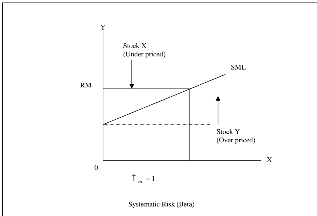
Figure 2.3 The security Market Line (SML)
