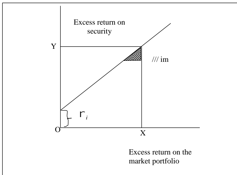
Figure 2.1:A security Characteristic Line
