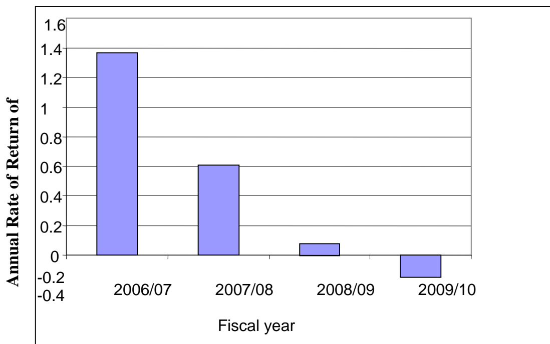
Figure 4 Annual Rate of Return of C.S. EBL
