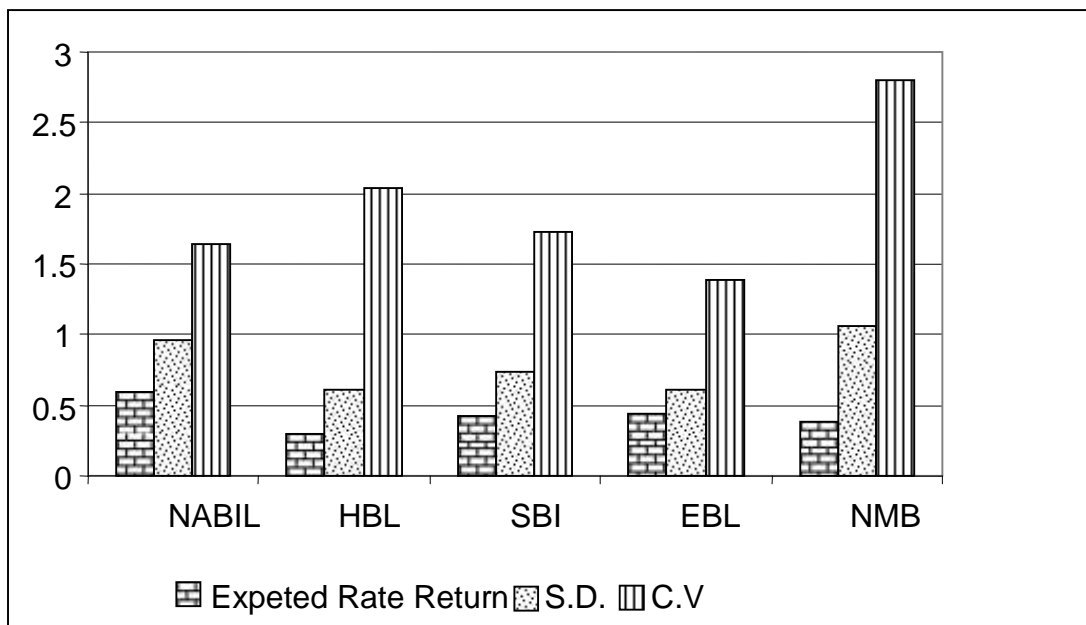
Figure 4.13 Expected Return, S.D. and C.V. of each Bank
