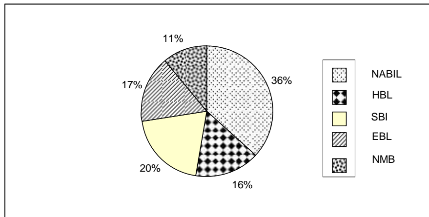
Figure 4.13 Comparative Proportion of Market Capitalization of Bank
