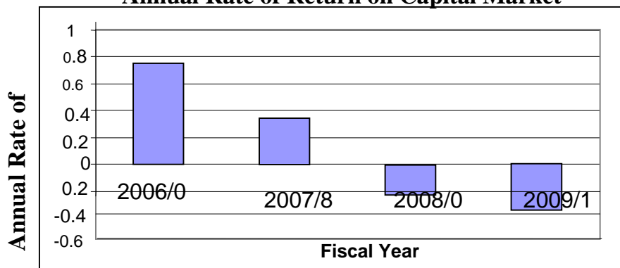
Figure 4.15 Annual Rate of Return on Capital Market
