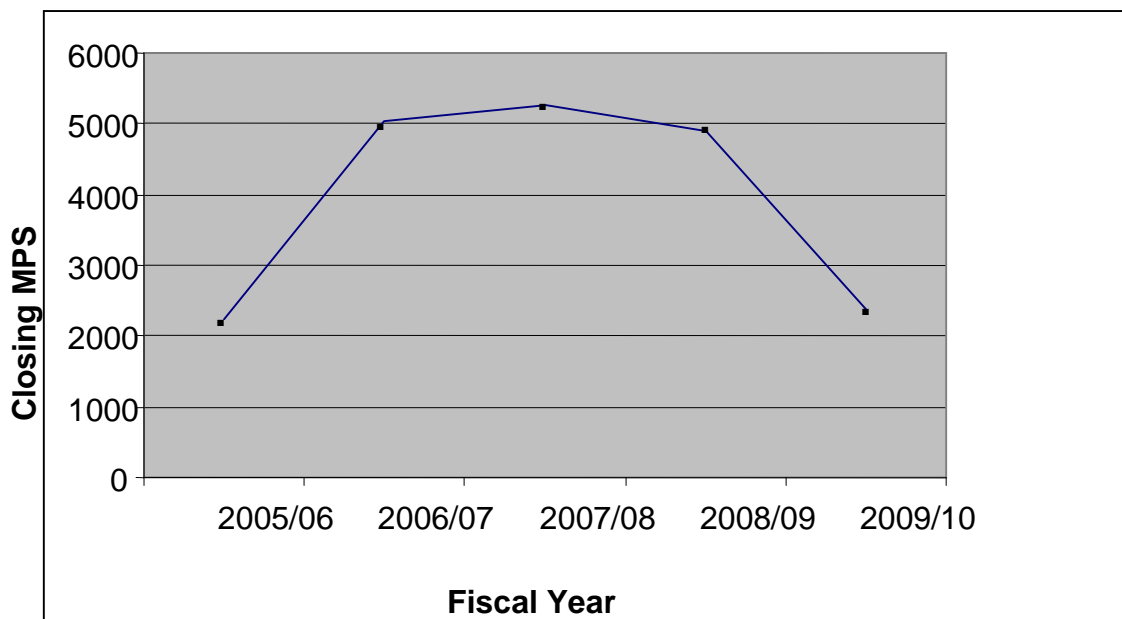
Figure 4.6 Market Price Movement of the C.S. of Nepal
