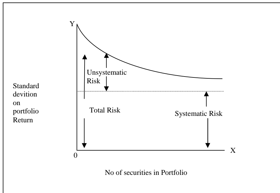
Figure 2.2 Portion of Risk on a portfolio
