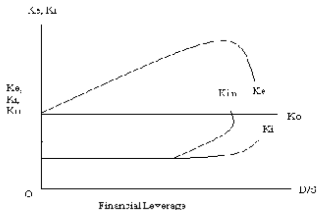
Figure 7: Behaviour of K_o , K_i and K_e under MM Hypothesis
