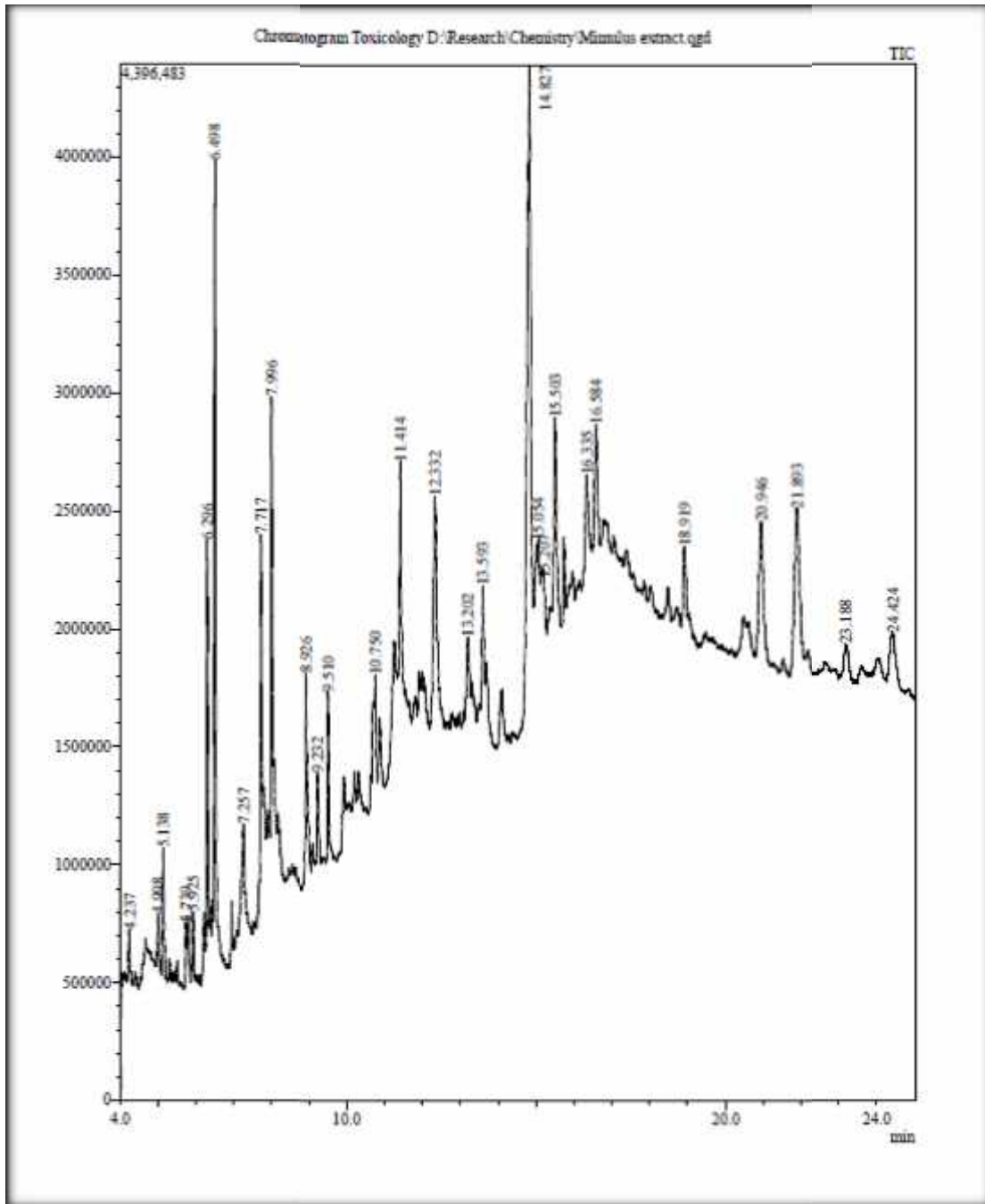
Figure 4.27GC-MS chromatogram of methanolic extracts of Mimulus nepalensis
