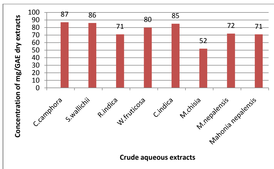
Figure4.8 Estimation of total phenol content of crude Aqueous extracts
