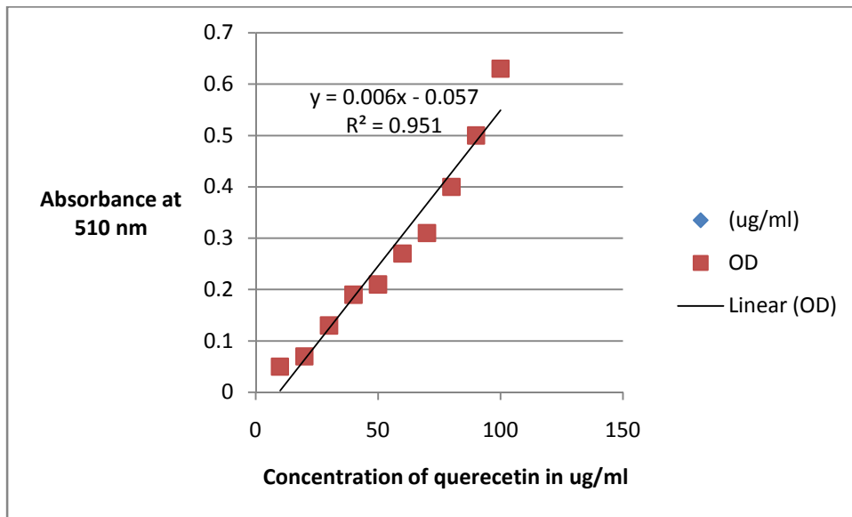
Figure 4.14 Standard of quercetin for aqueous extracts
