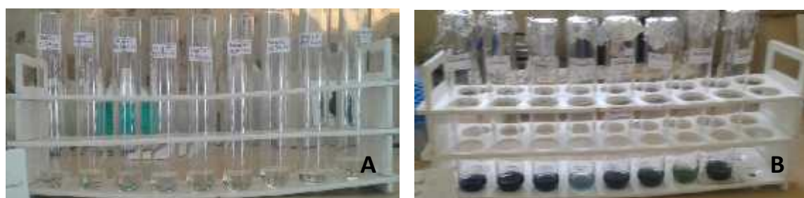
Figure4.9 Standard preparation of gallic acid and test of phenol test
