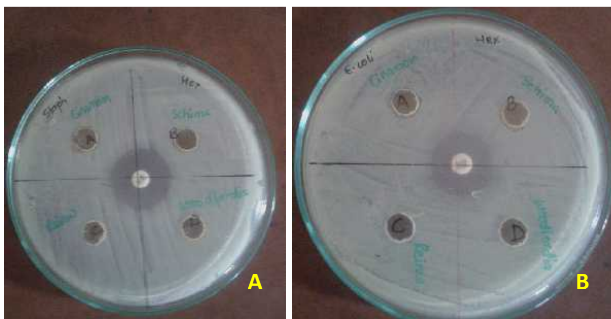
Figure 4.22 Hexane extracts of Plants in antibacterial tests
