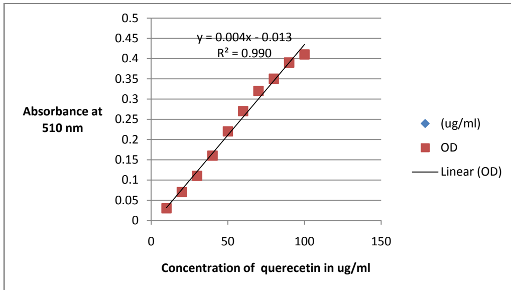
Figure 4.10 Standard of quercetin for ethyl acetate
