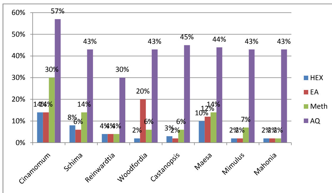
Figure 4.1 Percentage yield of plants extracts in different solvent
