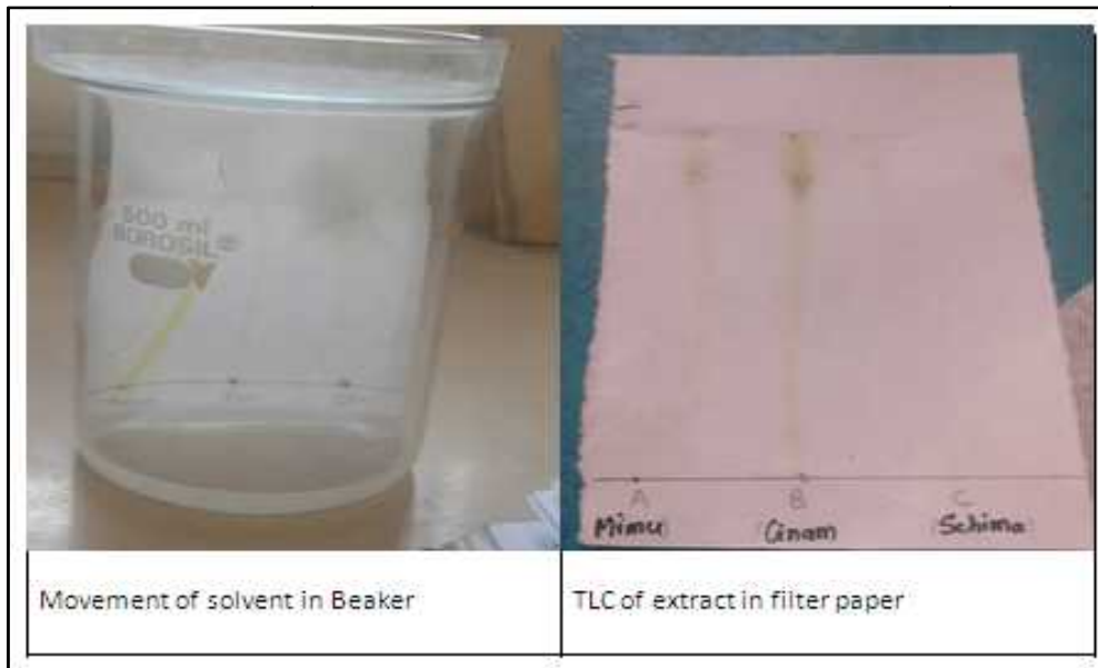
Figure 4.28TLC of plants extracts
