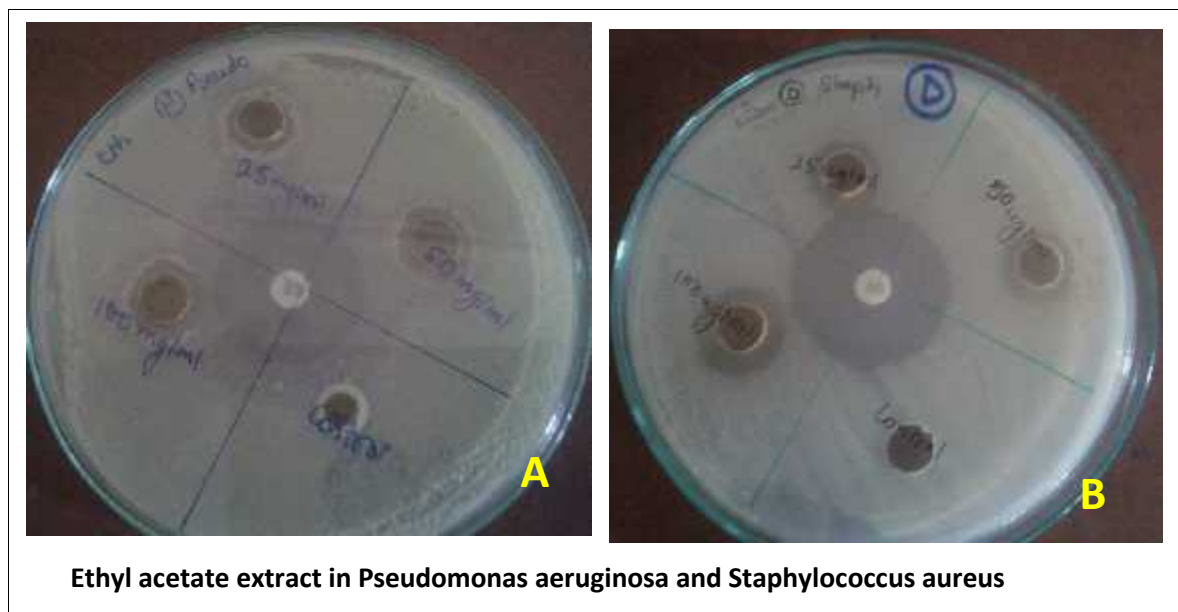
Figure 4.23 Ethyl acetate extracts in antibacterial test
