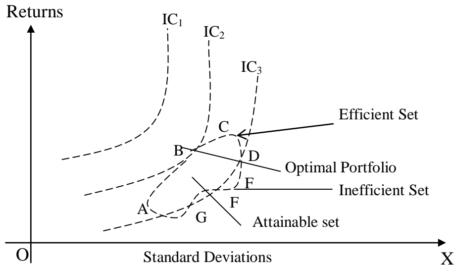
Figure 2.1 Portfolio Construction
