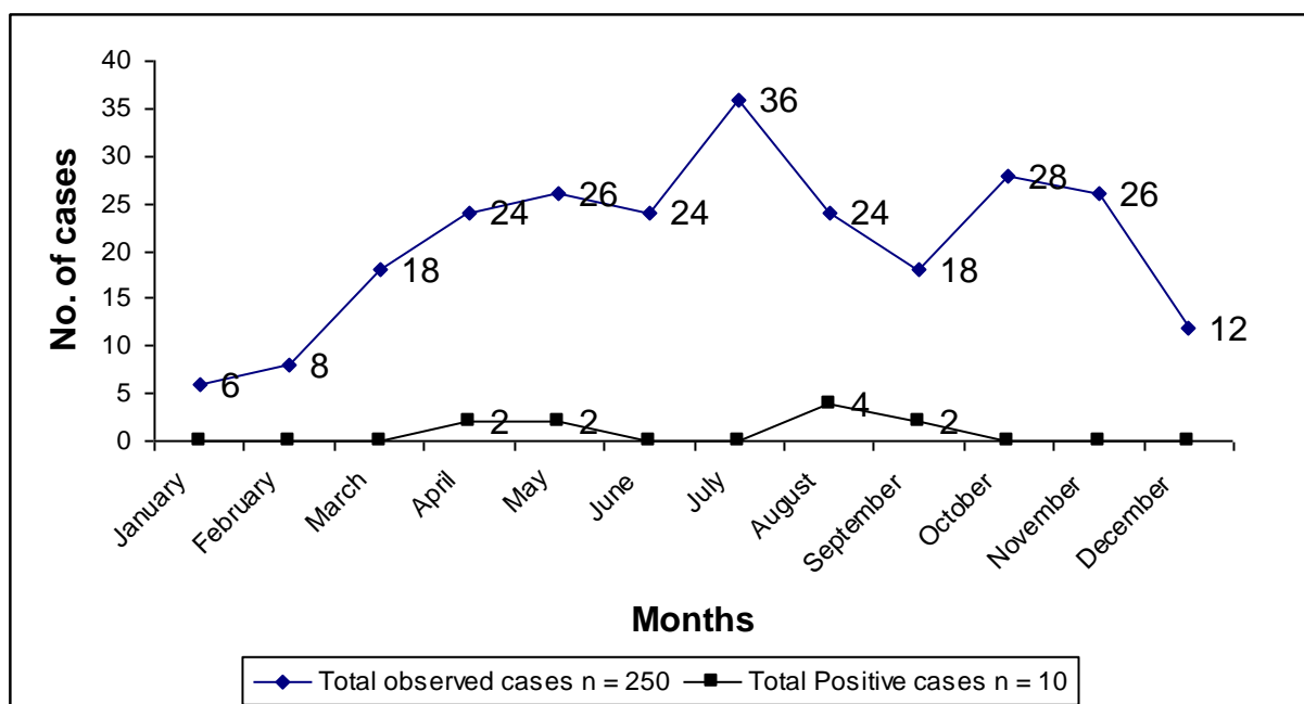
Figure 7: Month wise prevalence of malaria
