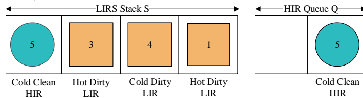
(g) State at Virtual Time 7
