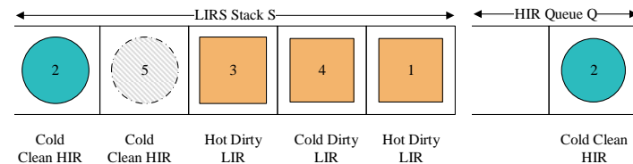
(h) State at Virtual Time 8
