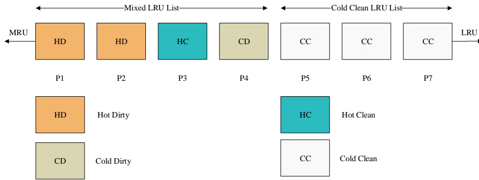
Figure 3.7: An example of CCF-LRU
