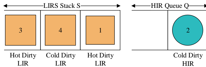
(f) State at Virtual Time 6
